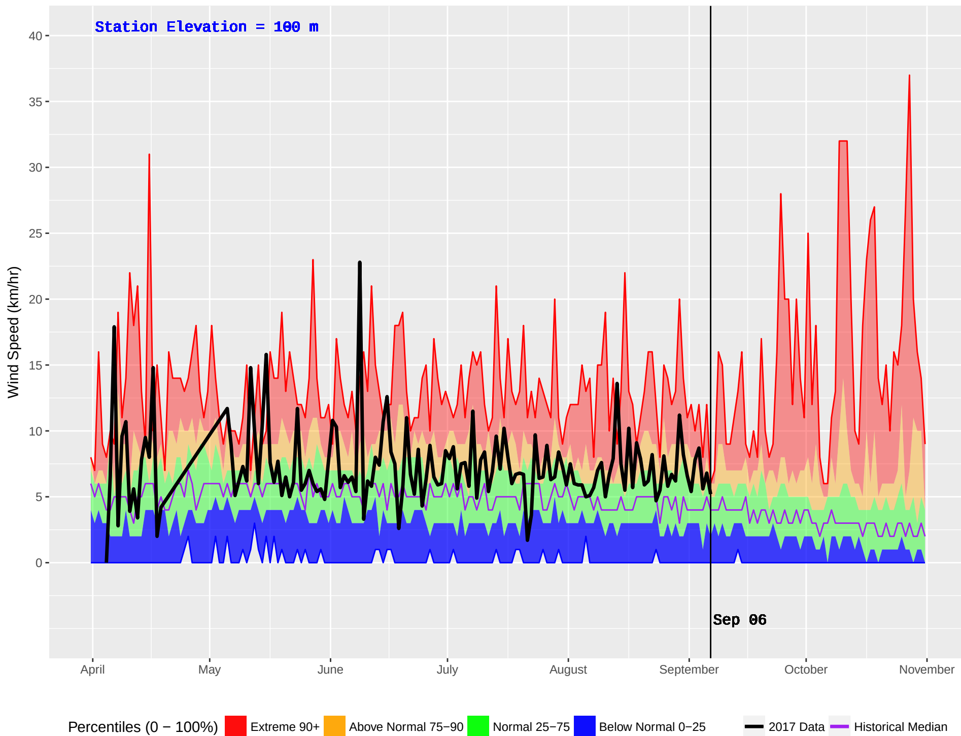
BEAVER CREEK (37) : Historical (1987–2016) and Current (2017) Noon Wind Speed
