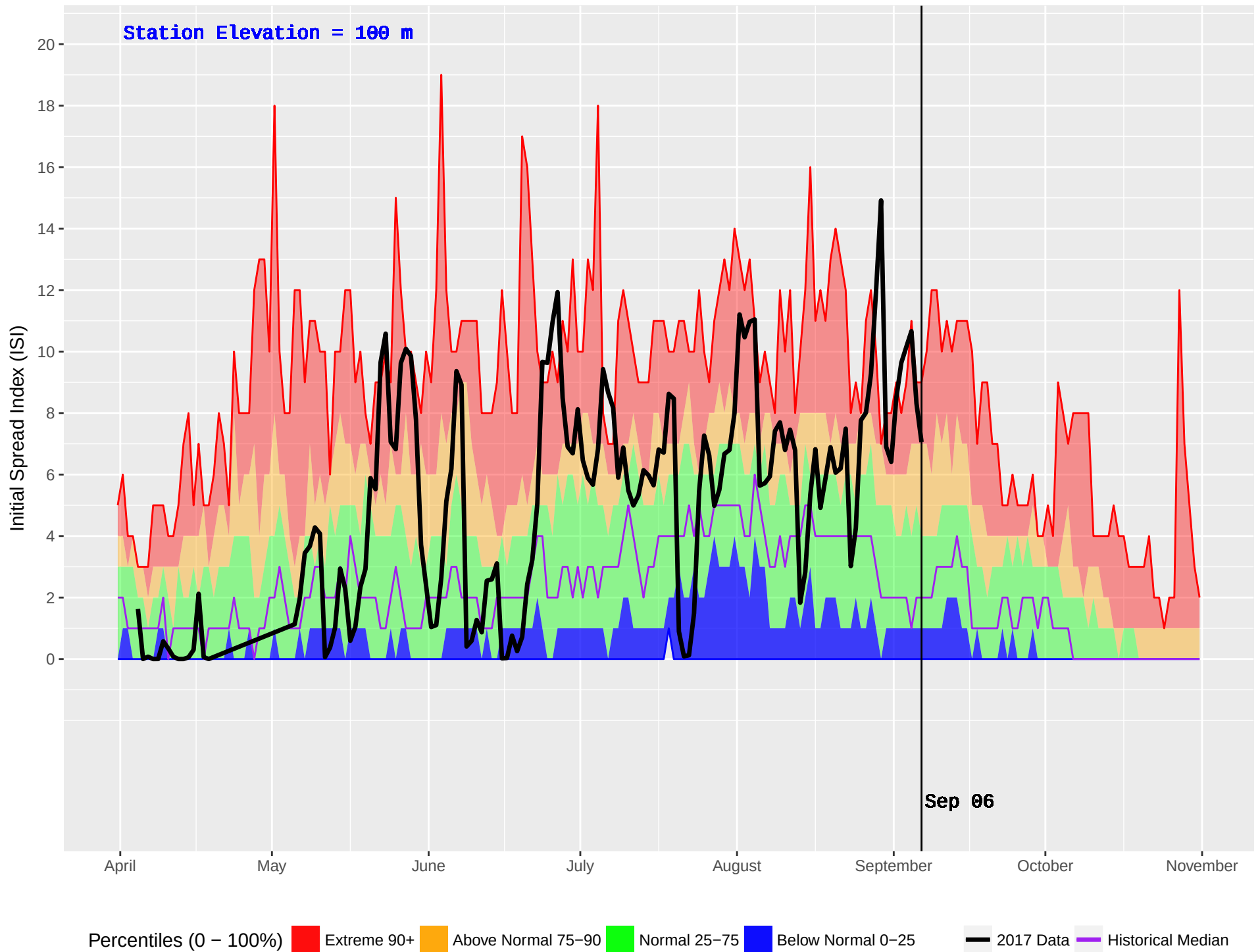
BEAVER CREEK (37) : Historical (1987–2016) and Current (2017) Noon Initial Spread Index (ISI)
